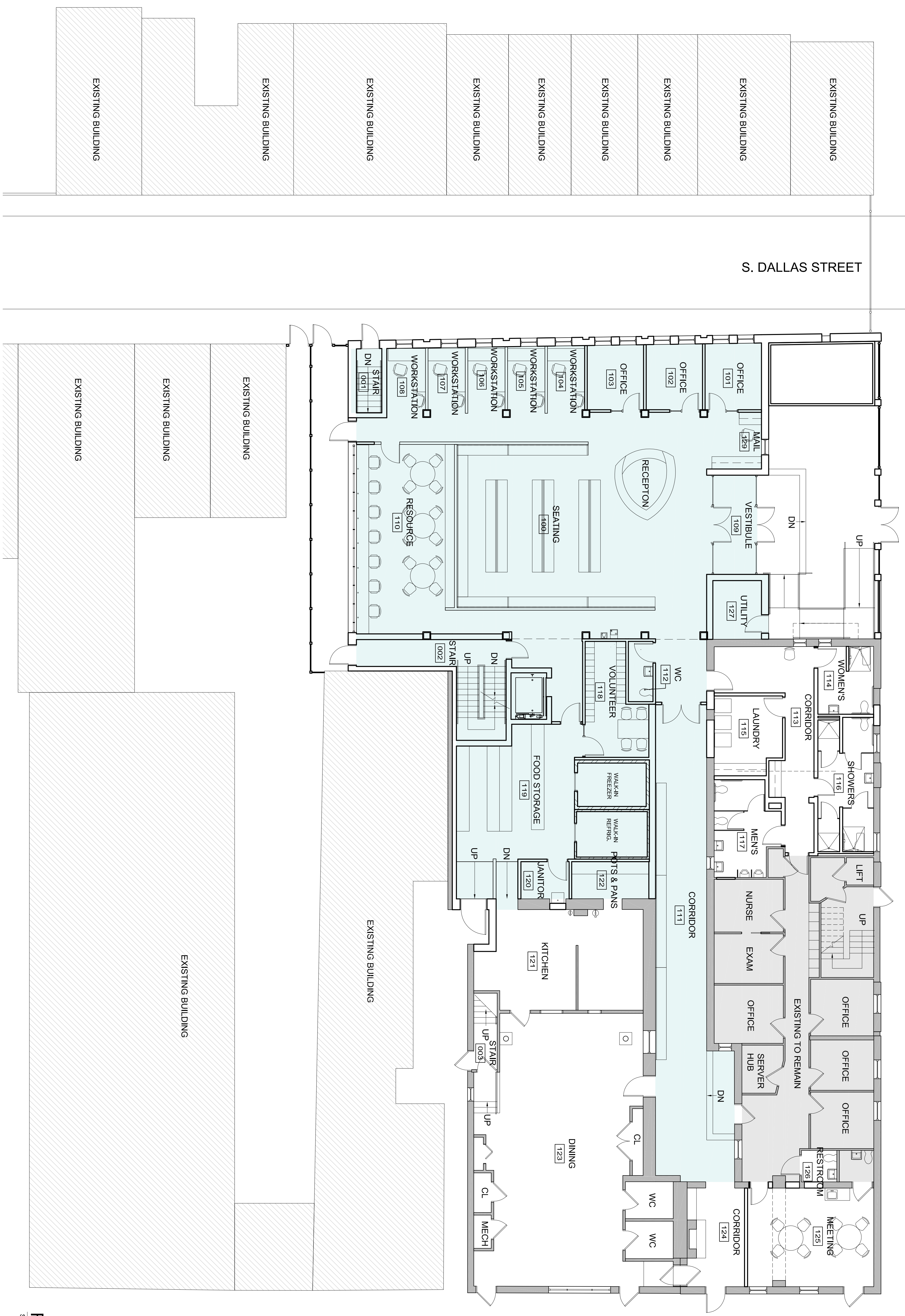
FIRST FLOOR PLAN SCALE 1/8" = 1'-0"
